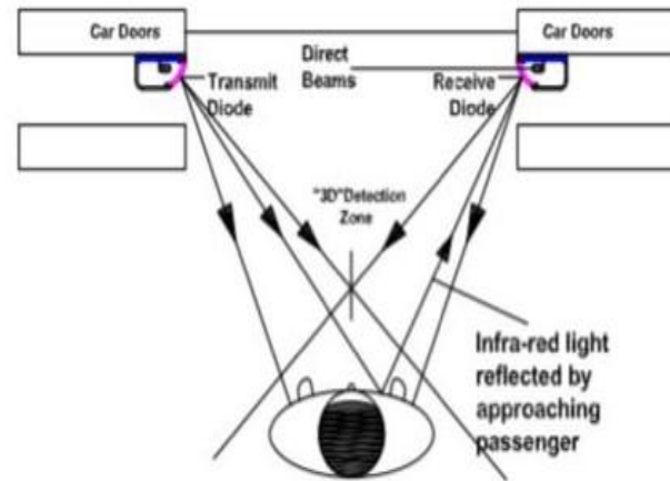
Fig 1 - The operating principle of the "3D" showing the sensitive zone projected into the landing
