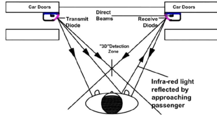
Fig 1 - The operating principle of the "3D" showing the sensitive zone projected into the landing
